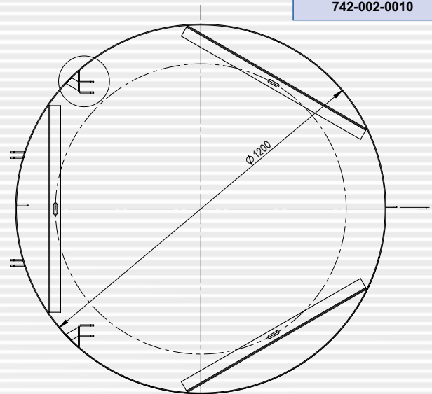
LPG sump, hot-dip galvanized 742-002-0010
