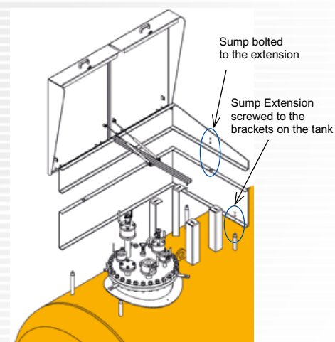
← Modular LPG INOX sump 231-190-0002
